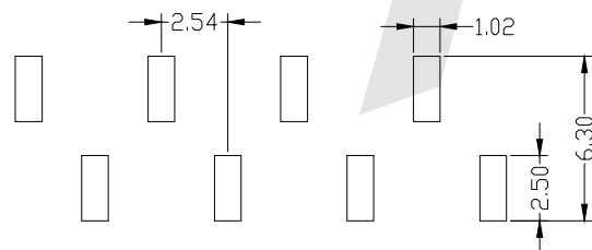
TYPE A PCB LAYOUT
