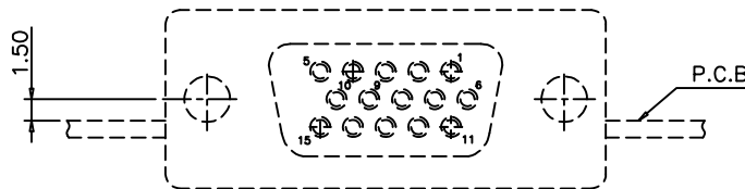
Recommended P.C.B Layout (component side)
